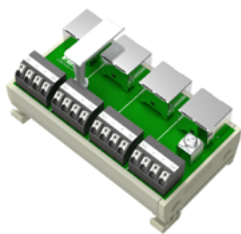
LT508-RJ45485-44PR (right connection)
