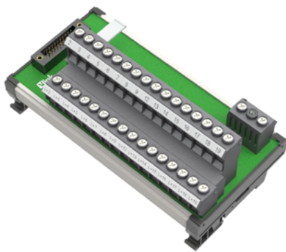
ST800-DI16SC-C 8.00Pitch
