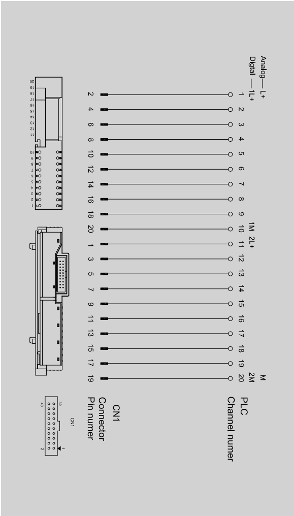
S7-300S-DA20P
