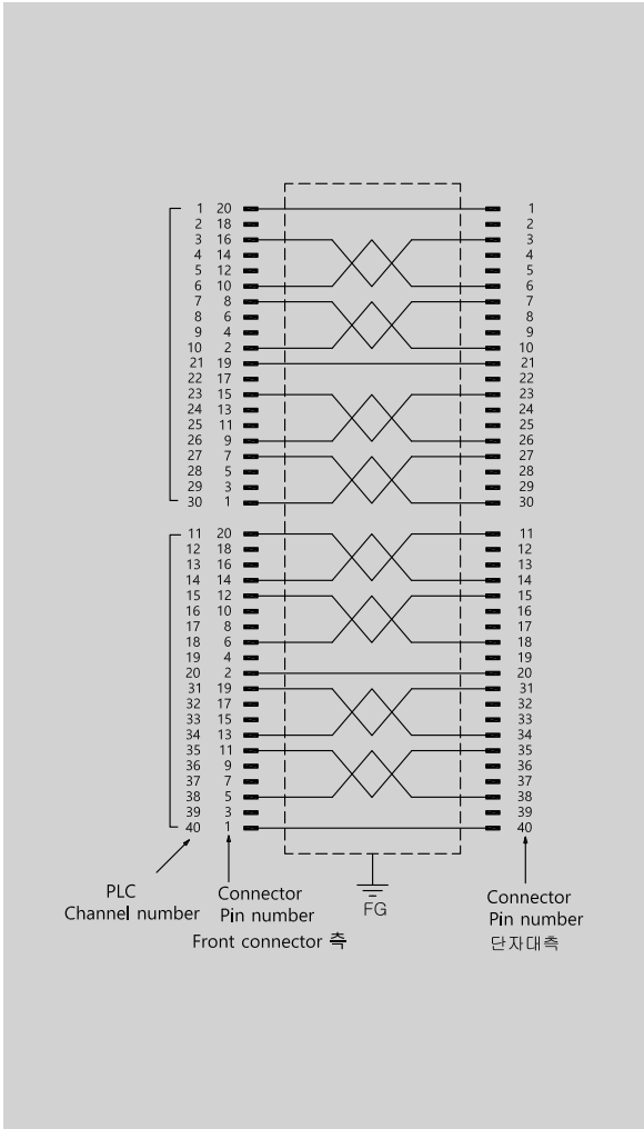
AHHC40-□K24BIS
