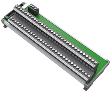
ST800-DI32SC-C 8.00 Pitch
